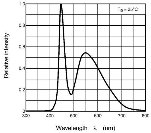
Fig. 8.4 Wavelength characteristic
